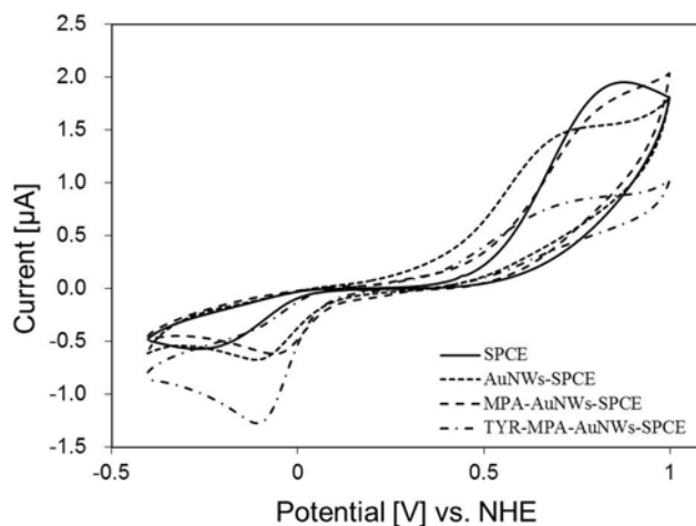
Fig. 4. The comparison of bare SPCE, AuNWs-SPCE, MPA-AuNWs-SPCE and TYR-MPA-AuNWs-SPCE for 1 mM of catechol in O_2 -saturated PBS (0.1 M, pH 7) at 50 \text{ mV s}^{-1} .
