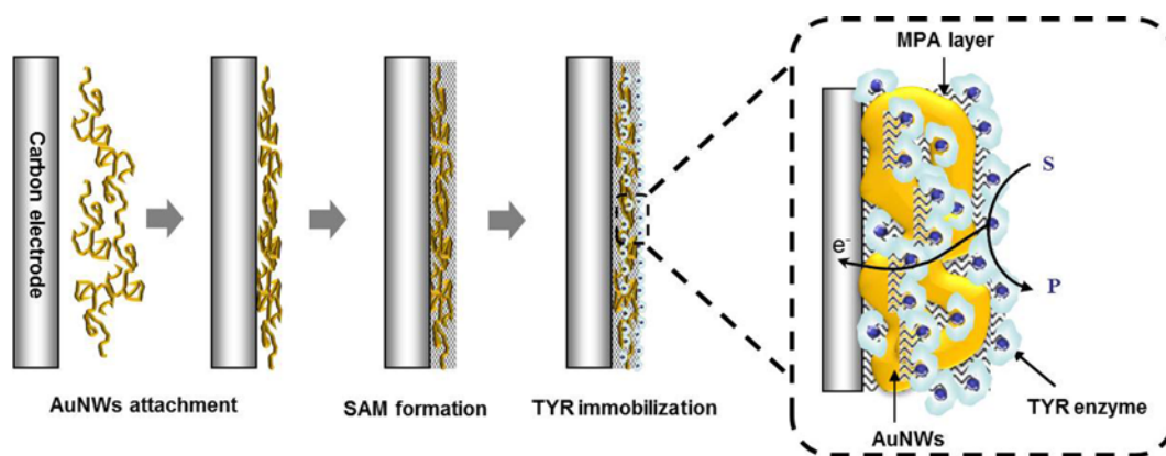
Fig. 1. Schematic diagram of the preparation of TYR-AuNWs-SPCE.
