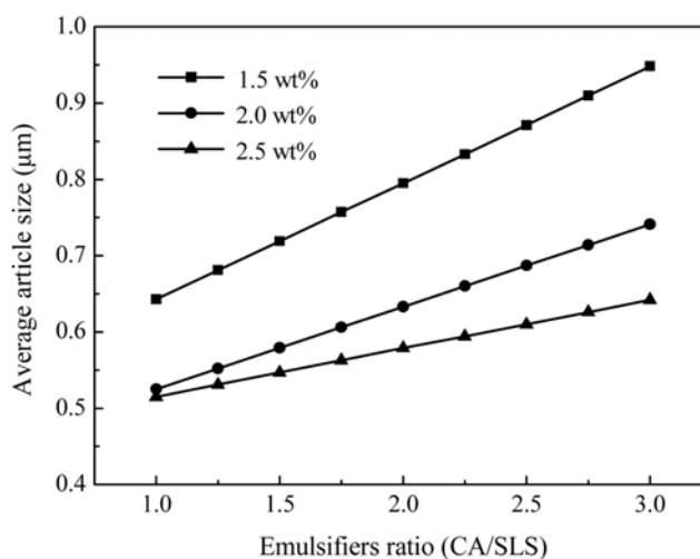
Fig. 4. The effect of the emulsifier ratio on the APS of PVC latex produced.
