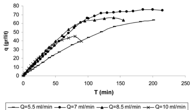
Fig. 3. Effect of feed flow rate on resin phase C=600 ppm T=25c Q (ml/min).
