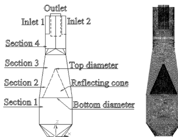
Fig. 1. Geometric model and mesh.
