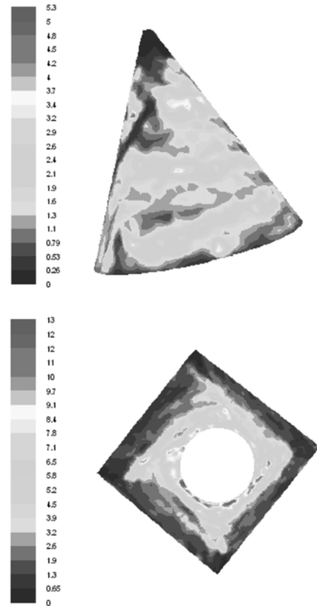
Fig. 12. Erosion at different parts of the separator.
