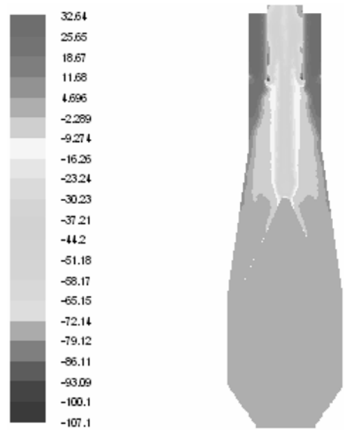
Fig. 5. Total pressure distribution.
