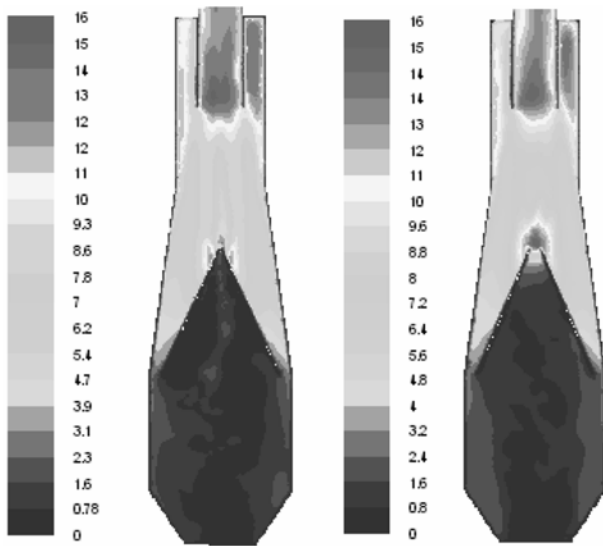
Fig. 10. Velocity graph with different top diameters.
