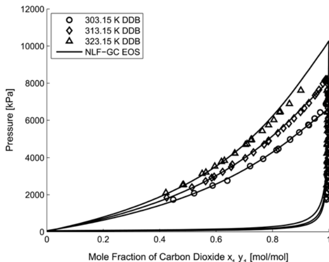
Fig. 5. Prediction results for the carbon dioxide+ethyl propionate system at different temperatures.
