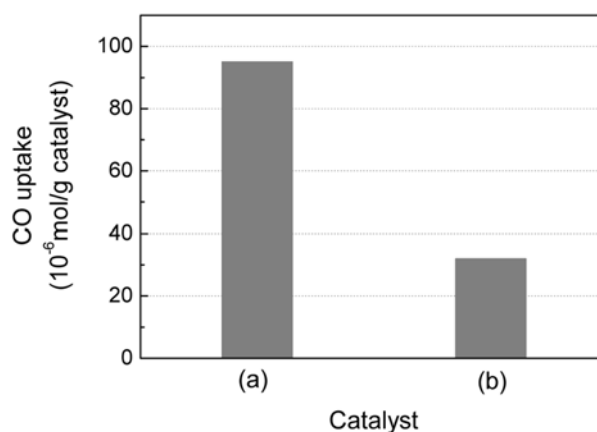
Fig. 3. CO uptake of Pt/CNT catalyst prepared by (a) ECD and (b) wet impregnation.
