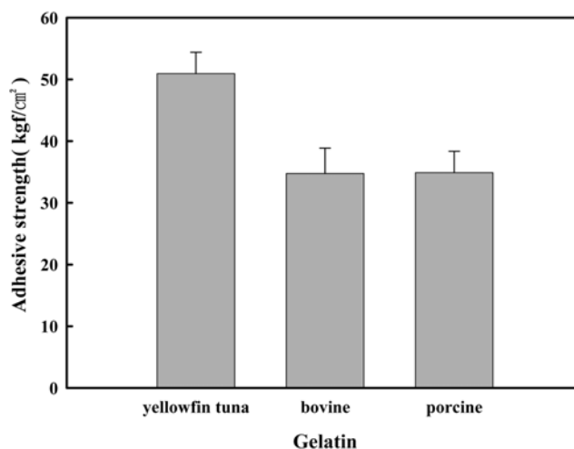
Fig. 3. Comparisons of adhesive strength of yellowfin tuna, bovine and porcine gelatins. The maturation was done at 22 \pm 1^\circ\text{C} for 25.68 hrs.
