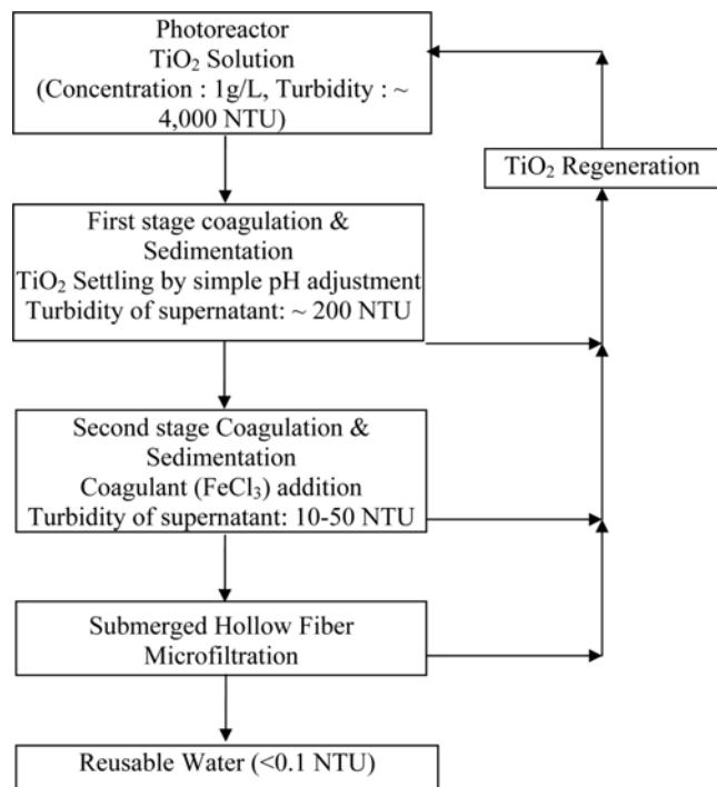
Fig. 9. Flow chart of post photocatalytic oxidation treatment for \text{TiO}_2 separation.
