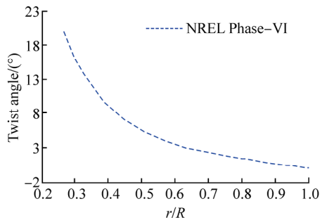
Fig. 1 Local twist angle along the blade
