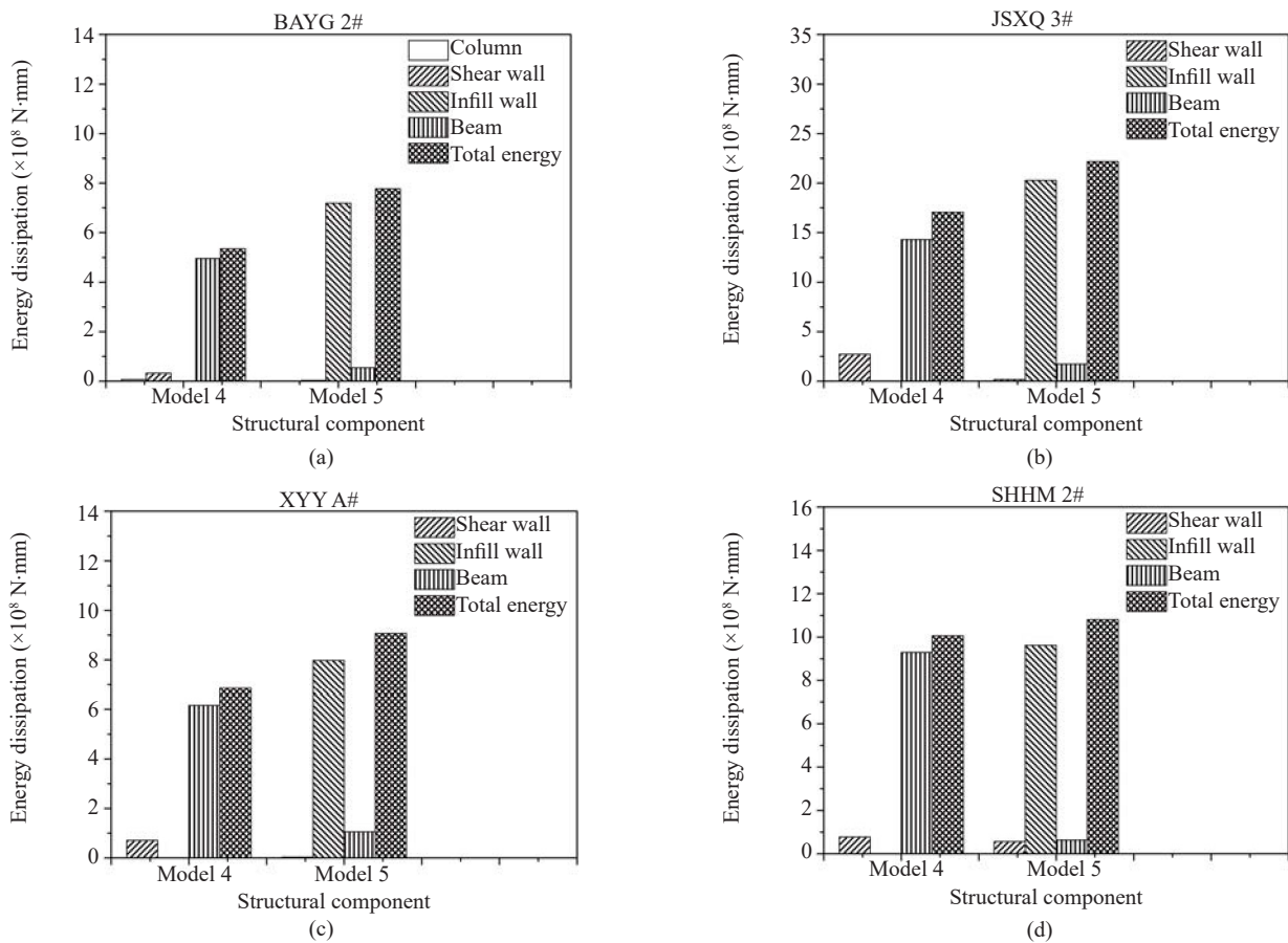
Fig. 21 Comparison of different members under large earthquakes: (a) BAYG 2#; (b) JSXQ 3#; (c) XYA A#; (d) SHHM 2#
