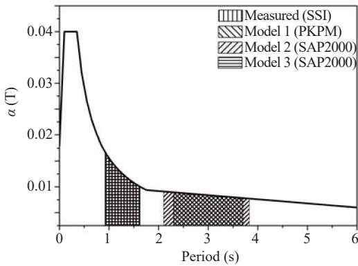
Fig. 13 Seismic influence factors in various analysis models
