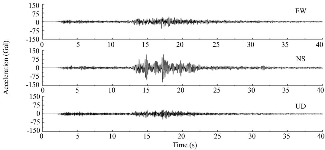
Fig. 10 Acceleration records obtained from Linjiaba gas station during the M 6.4 aftershock in Qingchuan (the epicenter distance is about 90 km). The PGAs in the EW, NS and UD directions are 58.8, 122.3 and 46.2 Gal, respectively
