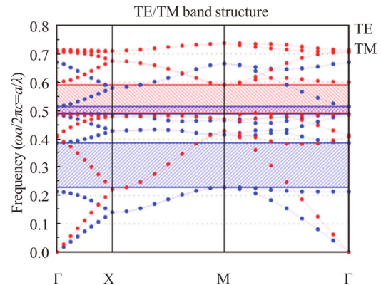
Fig.2 Schematic of PBG of the proposed structure
