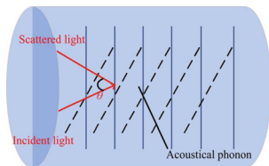
Fig.1 Schematic representation of SBS scattering in FMF
