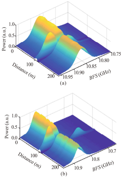
Fig.4 Normalized BGS at 60 °C for (a) SI-2-FMF and (b) SI-4-FMF
