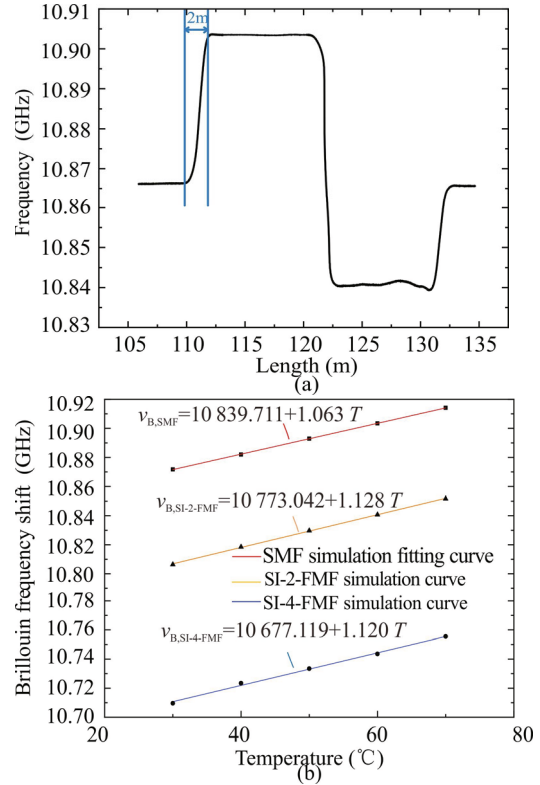
Fig.5 (a) BFS at 70 °C; (b) Temperature coefficient fitting curves
