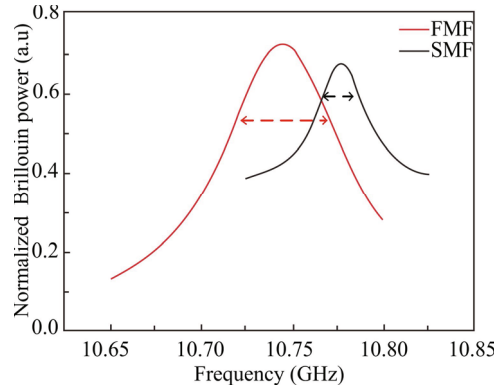
Fig.2 Brillouin gain spectra of MMF and SMF
