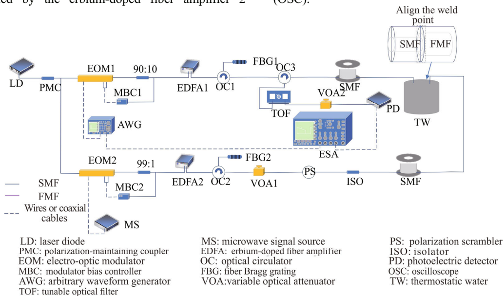
Fig.3 Block diagram of the lossy external microwave modulation BOTDA system
