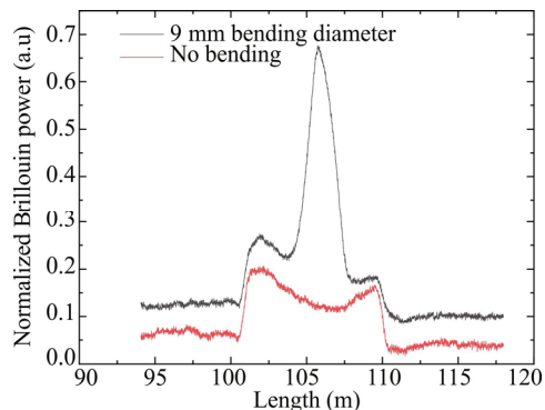
Fig.7 Normalized Brillouin power at 10.69 GHz
