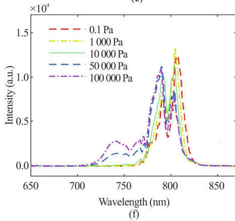
Fig.3 Transmitted spectra of the focused femtosecond pulses whose energy is (a, c, e) 2.48 mJ and (b, d, f) 0.74 mJ at different air pressures measured when (a, b) BF 1 + NF, (c, d) BF 2 + NF, and (e, f) NF are used
