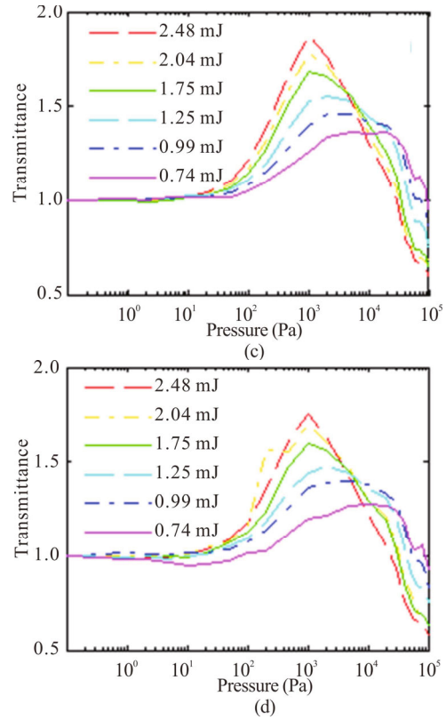
Fig.5 Energy transmittance of the 800 nm femtosecond pulses with air pressure when (a, b) BF 1 and (c, d) BF 2 are used ((a, c) and (b, d) are measured by the spectrographic and photoelectric methods, respectively)
