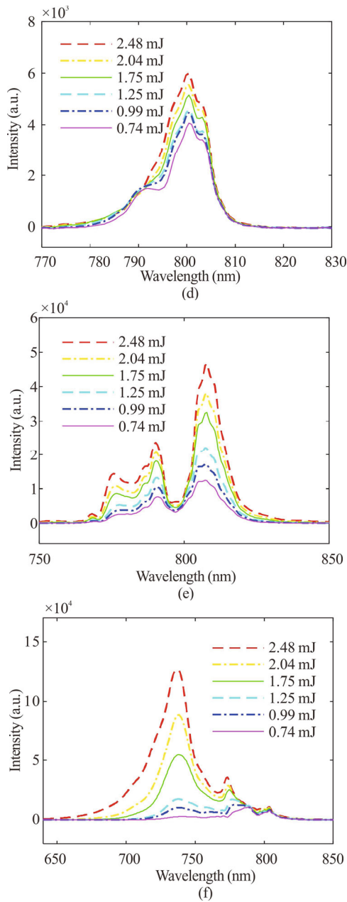
Fig.2 Transmitted spectra of the focused femtosecond pulses with different initial energies at (a, c, e) 0.1 Pa and (b, d, f) 100 kPa when (a, b) BF 1 (790—820 nm) + NF (740—865 nm), (c, d) BF 2 (795—805 nm) + NF and (e, f) NF are used
