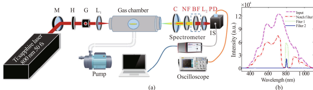
Laser: femtosecond laser; M: mirror; H: half-wave plate; G: Glan prism; L_1 , L_2 : focusing lenses; C: collimation lens; NF: notch filter; BF: band-pass filter; IS: integrating sphere; PD: silicon photodiode
