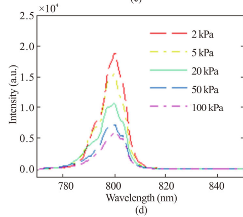
Fig.4 Transmitted spectra of the focused femtosecond pulses at different air pressures when (a, b) BF 1 + NF and (c, d) BF 2 + NF are used (The pulse energy is 2.48 mJ)
