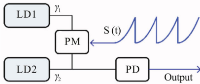
LD: laser diode; PM: phase modulator; PD: photodetector
