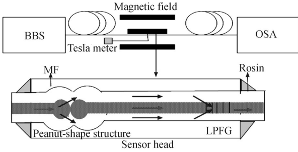
Fig.1 Schematic diagram of the experimental setup and the sensor structure
