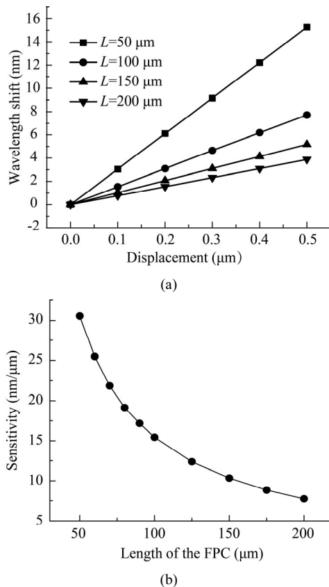
Fig.3 (a) Wavelength shift as a function of the displacement with different original L ; (b) Sensitivities of the FPI with various lengths of the FPC
