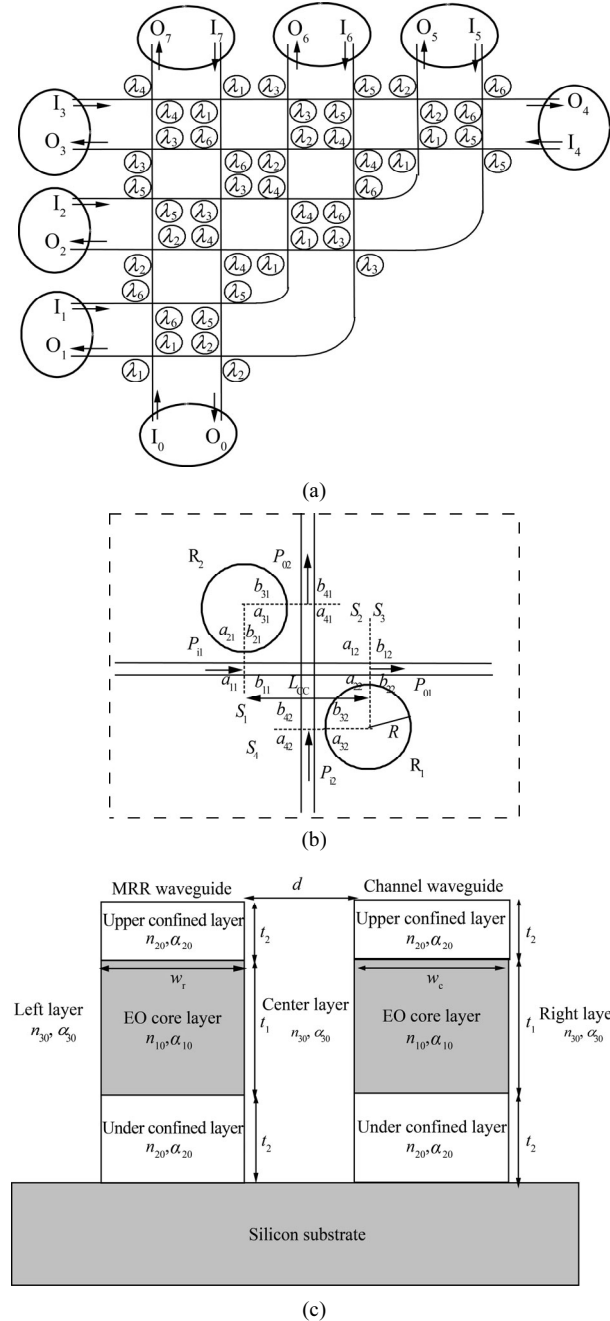
Fig.1 (a) Structure of the one-stage polymer 8-port optical router; (b) Structure of the polymer cross-coupling two-microring resonator; (c) Cross-section view over the coupling region between MRR waveguide and channel waveguide
