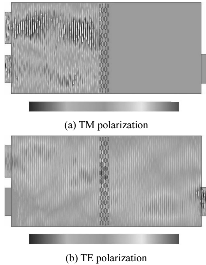
Fig.3 Steady-state electric field distributions at f=1.881 THz
