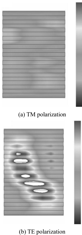
Fig.4 Steady-state electric field distributions in cross section at f=1.881 THz
