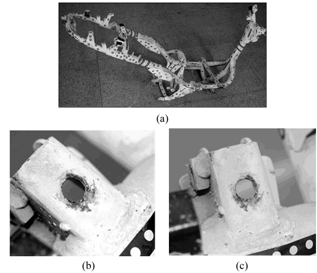
Fig.3 (a) Image of motorcycle frame; (b) Frame hole image from left camera; (c) Frame hole image from right camera
