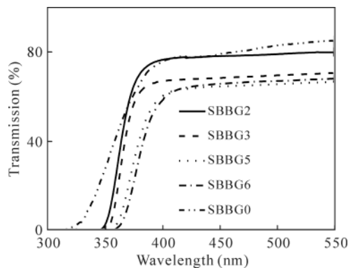
Fig.2 Transmission spectra of doped glasses with different amounts of Gd 2 O 3 and glass base
