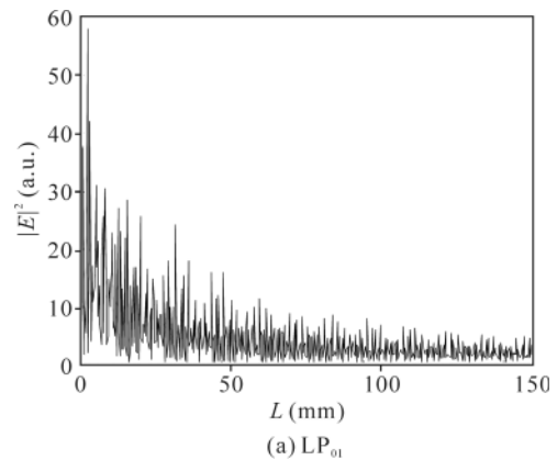
Fig.3 Output power for LP_{01} and LP_{11} modes versus propagation distance when Q=30 \mu\text{m}
