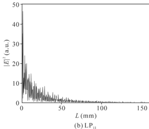
Fig.4 Output power for LP_{01} and LP_{11} modes versus propagation distance when Q=40 \mu\text{m}
