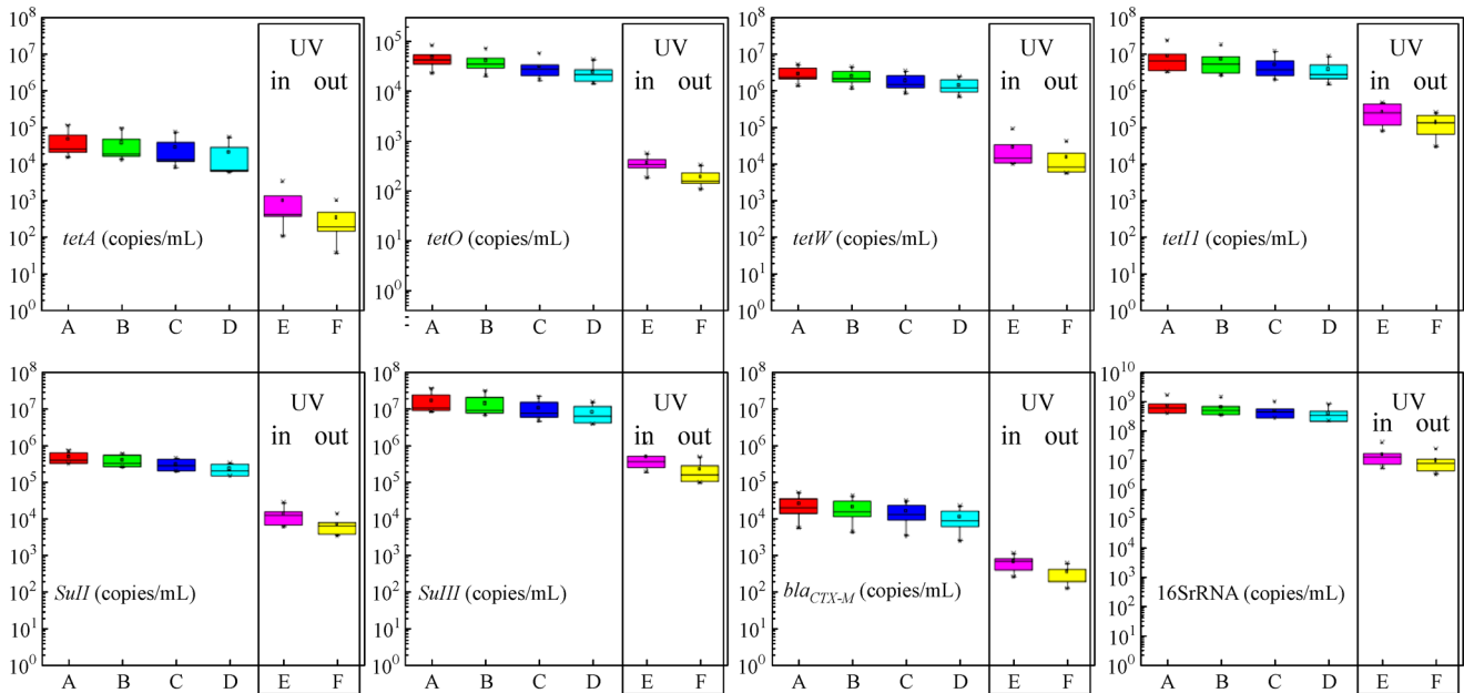
Fig. 2 Distribution of ARGs in the wastewater under different treatment processes (A, B, C, D, E, F represent the sampling locations after the coarse screen, the fine screen, the grit chamber, the sedimentation tank, CASS, and UV disinfection, respectively).
