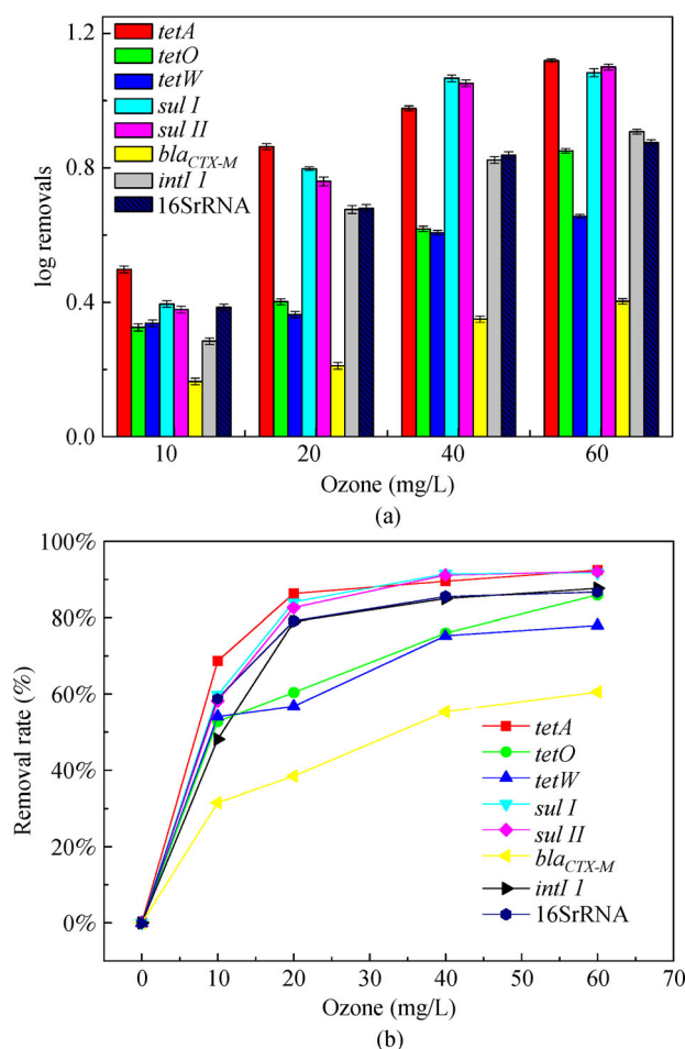
Fig. 4 Removal of ARGs by ozone disinfection.
