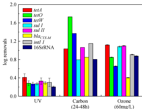
Fig. 6 Comparison of different advanced treatments for ARG removal.
