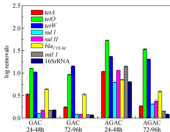
Fig. 5 Removal of ARGs by activated carbon treatments
