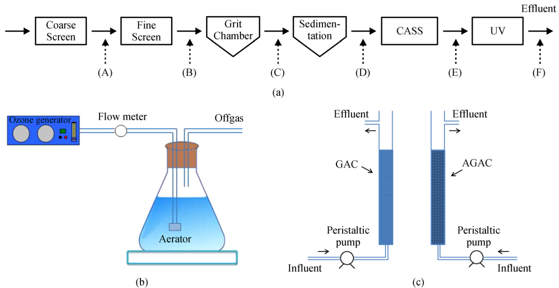
Fig. 1 (a) WWTP processes and sampling sites: (A) after the coarse screen, (B) after the fine screen, (C) after the grit chamber, (D) after the sedimentation tank, (E) after CASS, and (F) after UV disinfection. Configuration of post-treatments: (b) Ozone disinfection, (c) Granular activated carbon.
