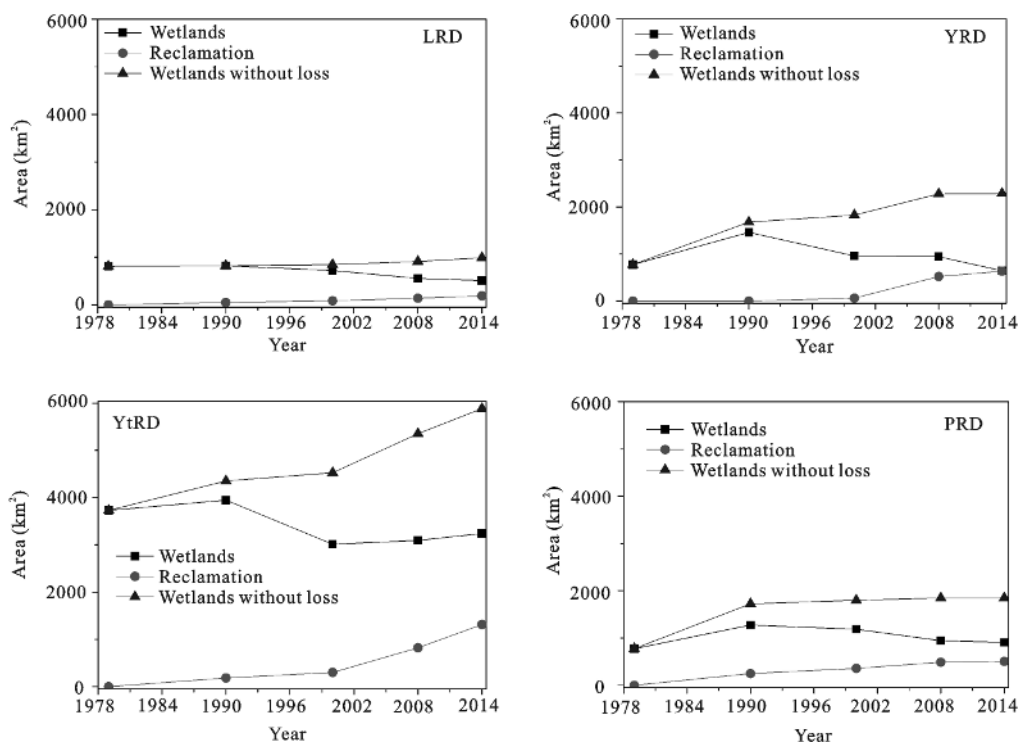
Fig. 2 Changes in the areas of coastal reclamation and natural wetlands in the four large river deltas during 1978–2014. LRD is the Liaohu River Delta; YRD is the Yellow River Delta; YtRD is the Yangtze River Delta; PRD is the Pearl River Delta
