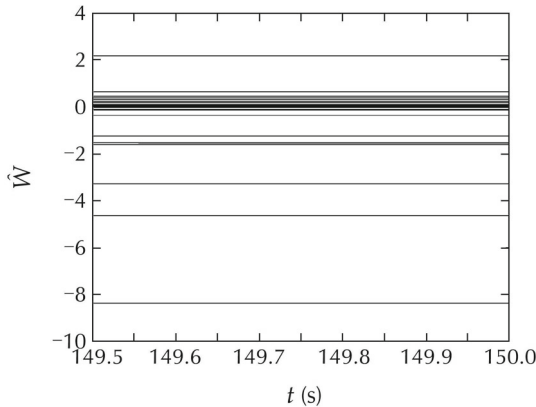
Fig. 3 Partial parameter convergence \hat{W} after the transient process. Each line corresponds to one neuron of the RBF network.
