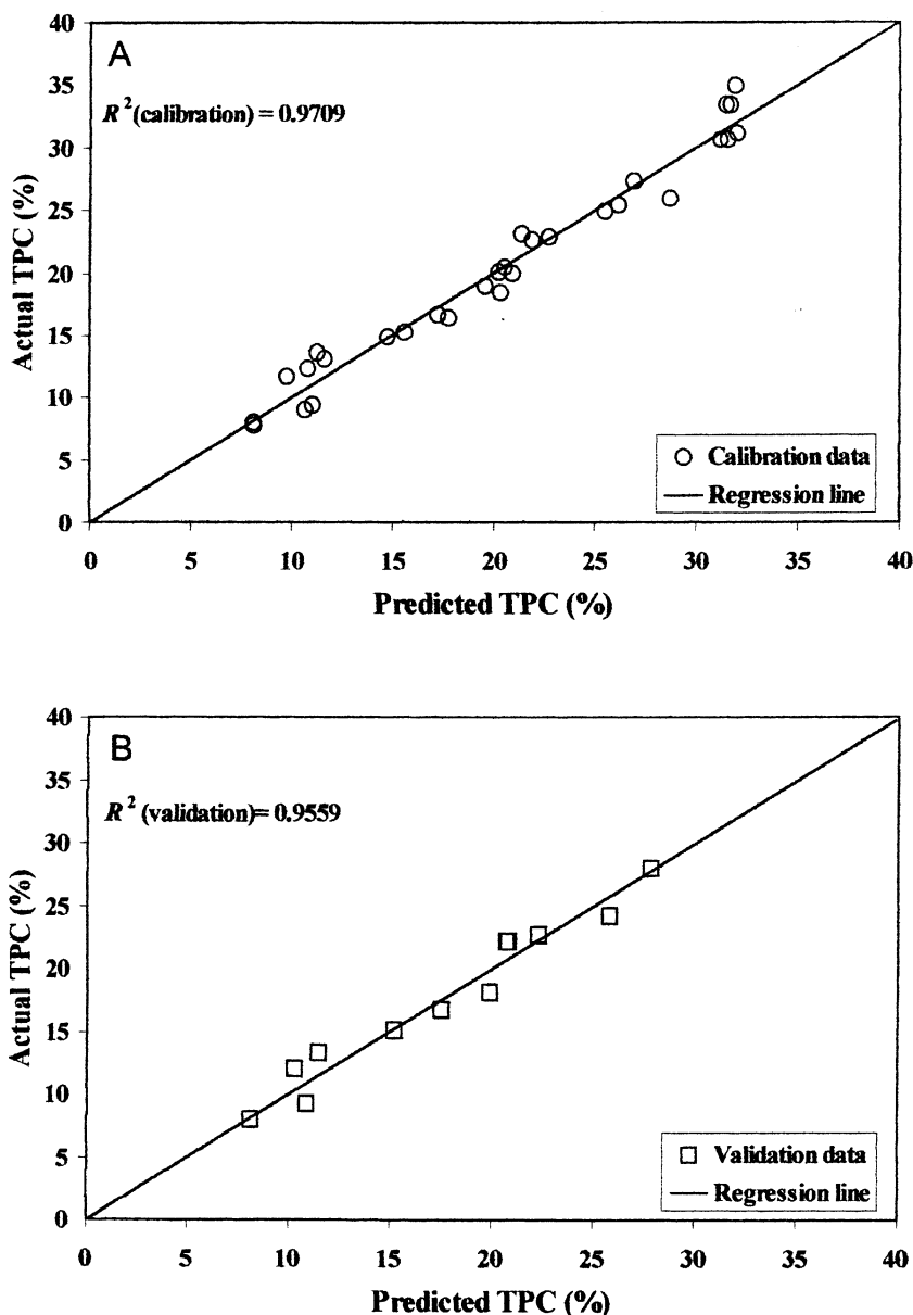
FIG. 7. Scatter plot showing calibration (A) and validation (B) data of actual vs. predicted TPC in percentage of RBDPO. Each value represents the mean of two independent determinations. For abbreviations see Figures 3, 5, and 6.
