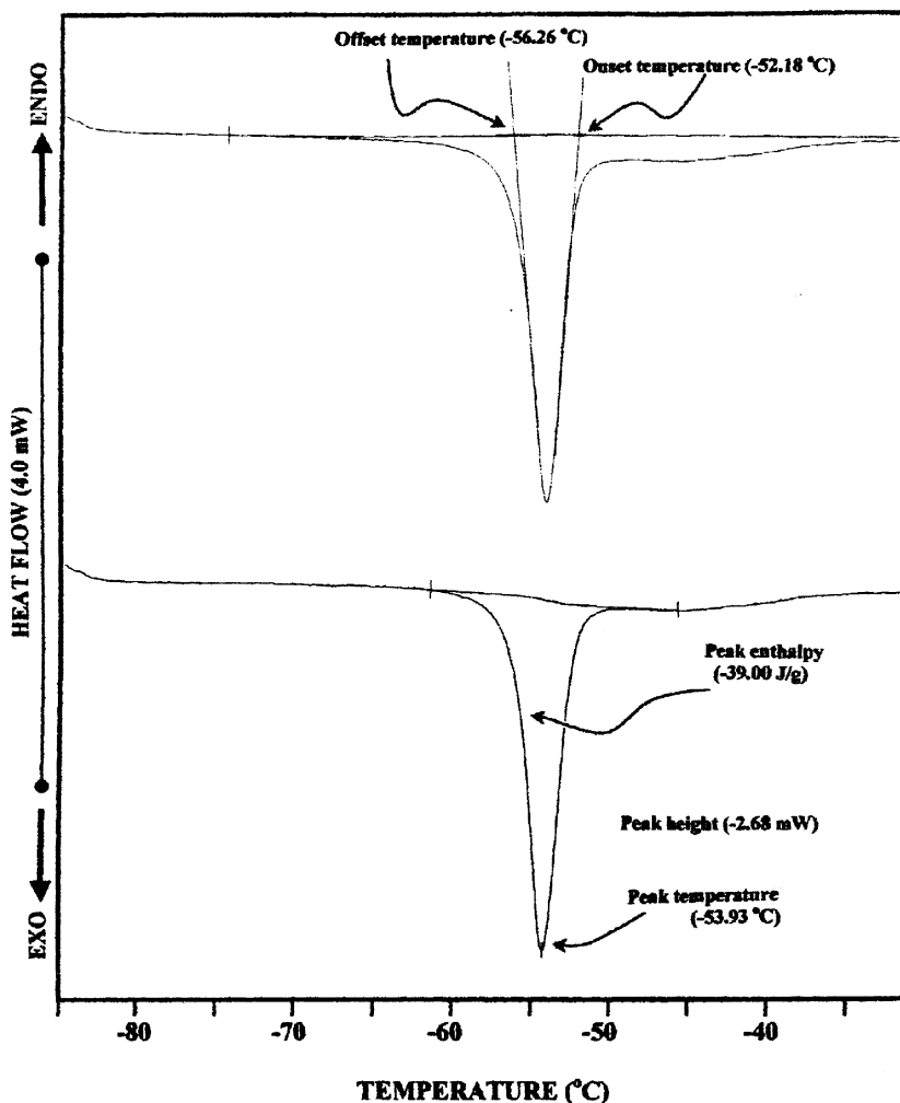
FIG. 1. Differential scanning calorimetry (DSC) cooling thermograms of corn oil. The techniques used for determination of the DSC parameters are illustrated by construction lines. (a) The onset and offset temperatures corresponded closely to the intersection of the extrapolated baseline and the tangent line (leading edge) of the peak. (b) A sigmoidal/curved baseline is constructed before the calculation of peak temperature, enthalpy and height by using 7 Series/UNIX software library (Perkin Elmer Corp., Norwalk, CT).
