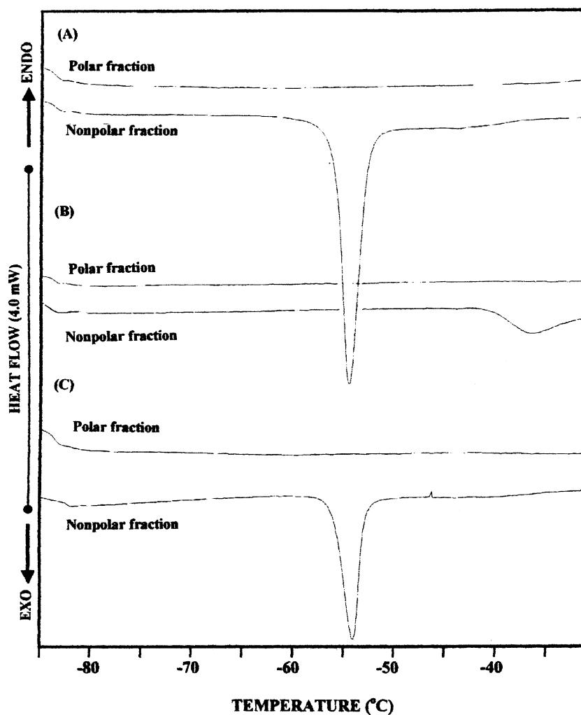
FIG. 5. Cooling thermograms of polar and nonpolar fraction of (A) corn oil sample with 23.84% TPC; (B) RBDPO sample with 19.97% TPC; and (C) soybean oil with 25.82% TPC. See Figures 2 and 3 for abbreviations.
