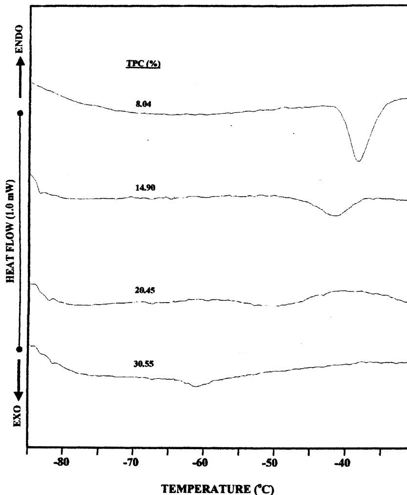
FIG. 3. Cooling thermograms of refined, bleached, and deodorized palm olein (RBDPO) samples with different concentrations (percentage) of TPC. See Figure 2 for abbreviation.
