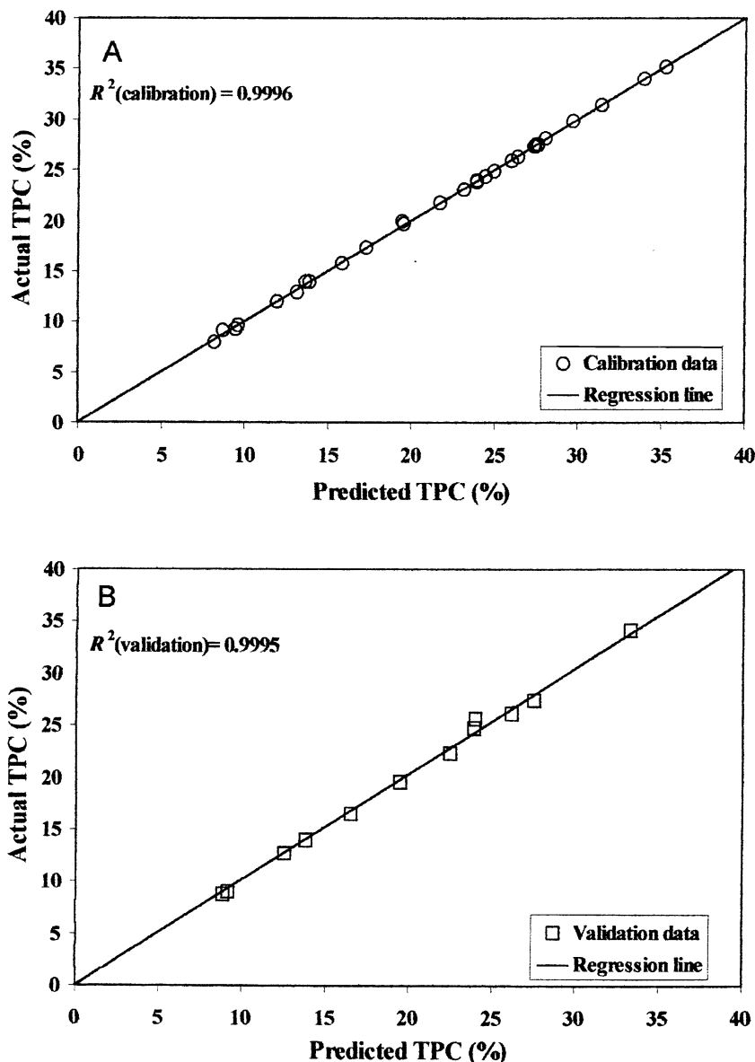
FIG. 6. Scatter plot showing calibration (A) and validation (B) data of actual vs. predicted TPC percentage of corn oil. Each value represents the mean of two independent determinations. R^2 , coefficient of determination; for other abbreviation see Figure 2.
