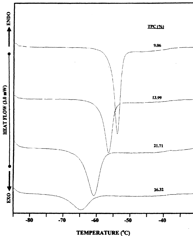
FIG. 2. Cooling thermograms of corn oil samples with different concentrations (percentage) of total polar compounds (TPC).
