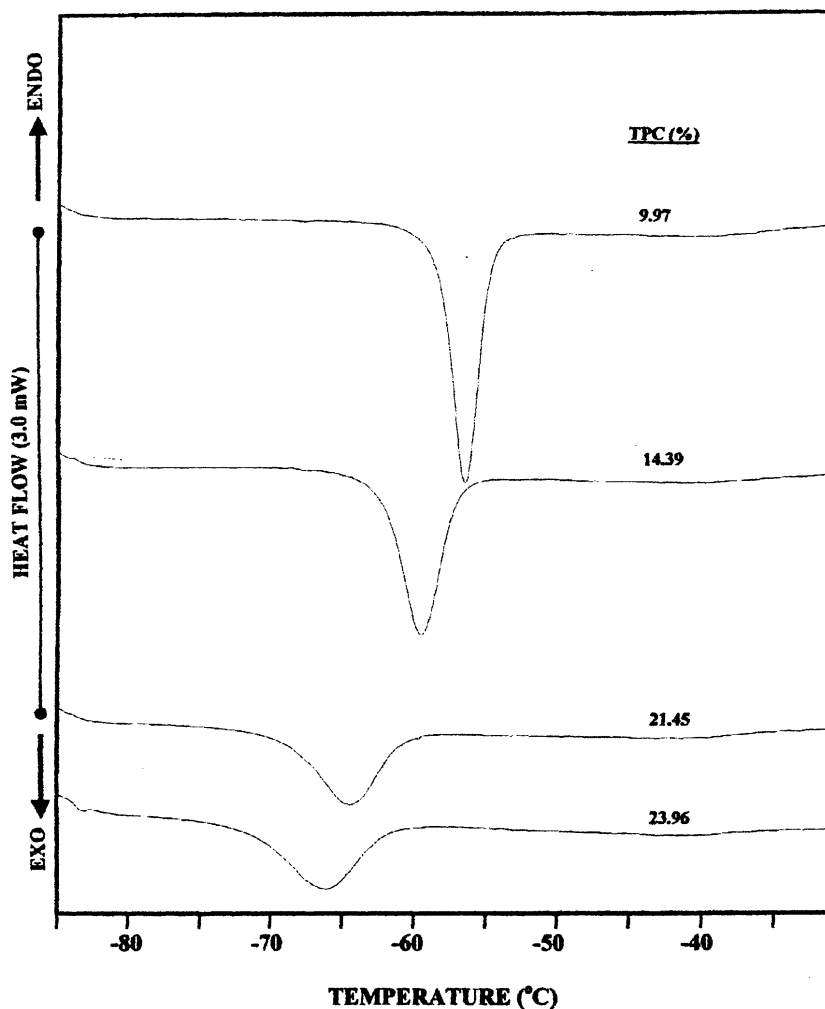
FIG. 4. Cooling thermograms of soybean oil samples with different concentration (percentage) of TPC. For abbreviation see Figure 2.
