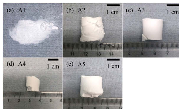
Fig. 1 MTMS-derived SAs via APD method while using (a) deionized water, (b) hexane, (c) 0.044 g·mL -1 sodium bicarbonate solution, (d) 0.022 g·mL -1 sodium bicarbonate solution in solvent exchange step, respectively along with (e) sample A3 after extra wash to remove salt, labelled as A5.
