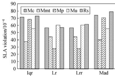
Fig. 3 SLA violations
