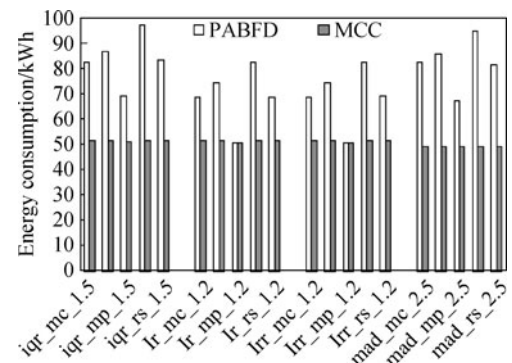
Fig. 7 Energy consumption MCC/PACFD
