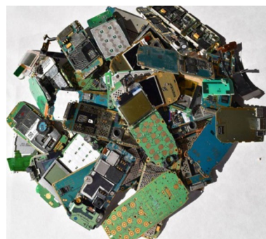
Fig. 1 PCBs of mobile phones
