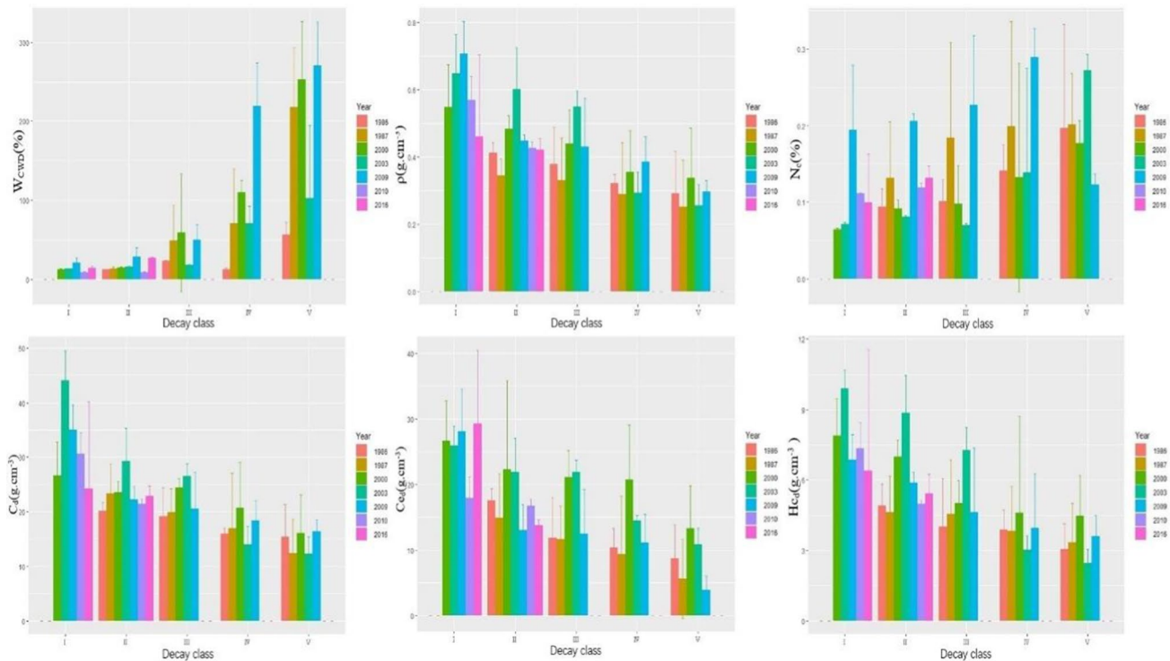
Fig. 3 Average value of variables in five decay classes in different burned patches; W_{CWD} , coarse wood debris water content; \rho , coarse wood debris density; N_c , nitrogen content; C_d , carbon density; Ce_d , cellulose density; Hc_d , hemicellulose density
