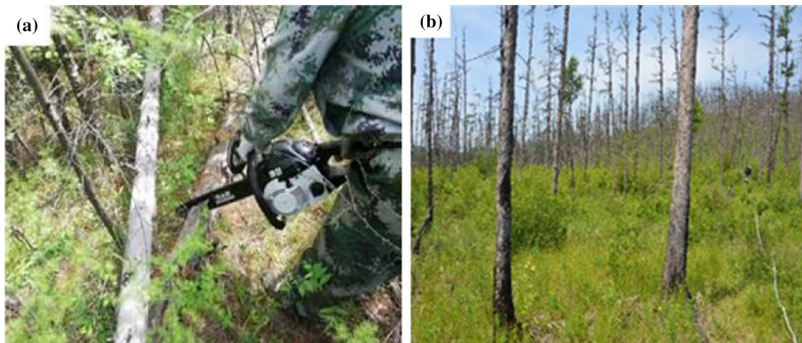
Fig. 2 Burned patches in the Greater Khingan Mountains in 2003 a and 2010 b
