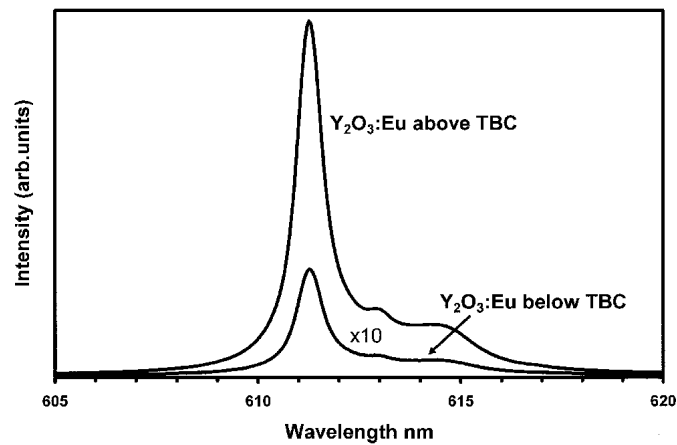
Fig. 6 Comparison of 611 nm emission intensity at room temperature for Y_2O_3:Eu layer above versus below freestanding 100 \mu m thick PS-8YSZ TBC; the emission spectrum for Y_2O_3:Eu below the TBC was multiplied 10 \times for easier comparison
