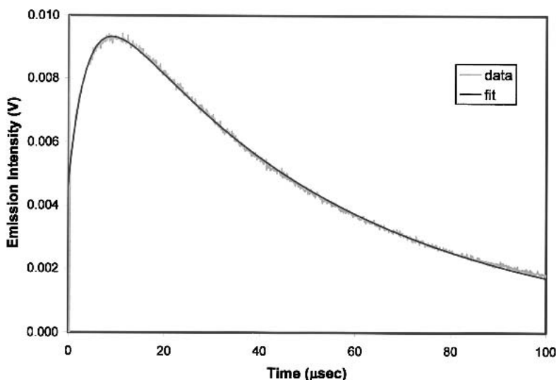
Fig. 3 Fluorescence decay curve at 700 °C from Y_2O_3:Eu layer beneath freestanding 100 \mu m thick PS-8YSZ (gray). The black curve is the result of fitting Eq 1 to the data.
