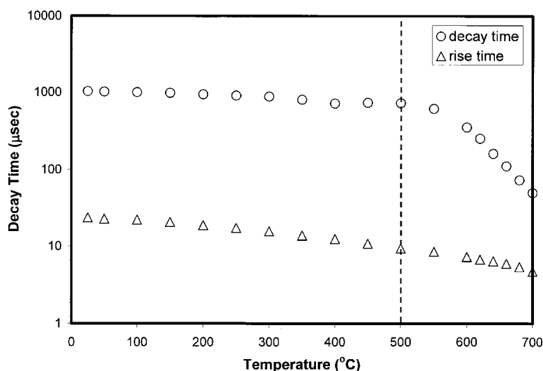
Fig. 8 Comparison of decay time ( \tau_{\text{decay}} ) versus rise time ( \tau_{\text{rise}} ) as a function of temperature determined from decay of 611 nm emission from \text{Y}_2\text{O}_3:\text{Eu} layer above freestanding 100 \mu\text{m} thick PS-8YSZ TBC
