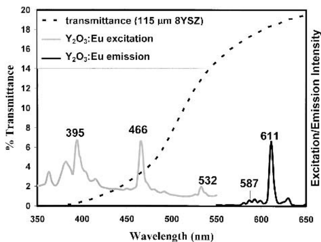
Fig. 1 Hemispherical transmittance plot for a 115 \mu\text{m} thick freestanding PS-8YSZ TBC along with excitation and emission spectra for \text{Y}_2\text{O}_3:\text{Eu}
