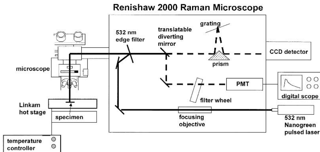
Fig. 2 Schematic illustration of the Raman-microscope-based system used to acquire both phosphor layer emission spectra and fluorescence decay time measurements as a function of coating temperature
