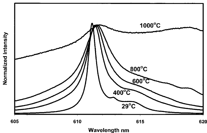
Fig. 4 Emission spectra as a function of temperature for Y_2O_3:Eu layer above freestanding 100 \mu m thick PS-8YSZ TBC
