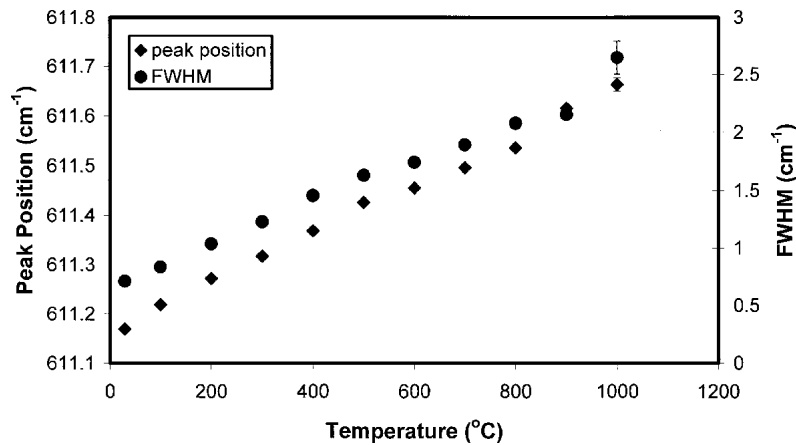
Fig. 5 Peak position and FWHM of 611 nm emission peak from Y_2O_3:Eu phosphor layer as a function of temperature
