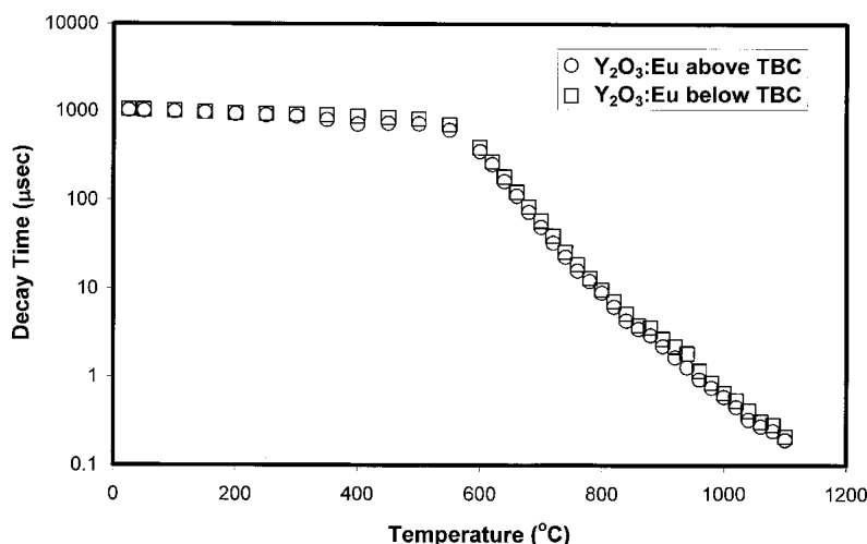
Fig. 7 Decay time ( \tau_{\text{decay}} ) as a function of coating temperature for \text{Y}_2\text{O}_3:\text{Eu} layer above versus below freestanding 100 \mu\text{m} thick PS-8YSZ TBC
