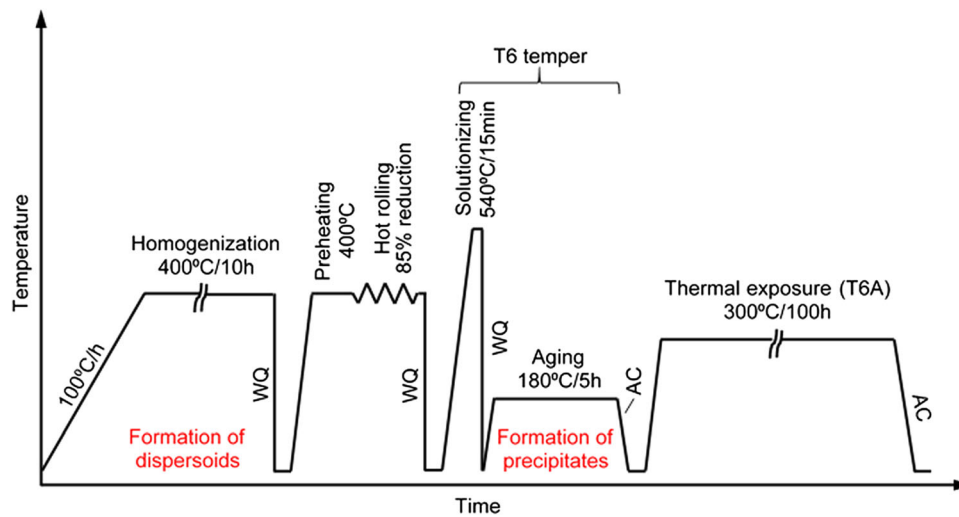
Fig. 1 Thermomechanical processing route of 6082 alloy sheets. WQ and AC refer to water quenching and air-cooling, respectively
