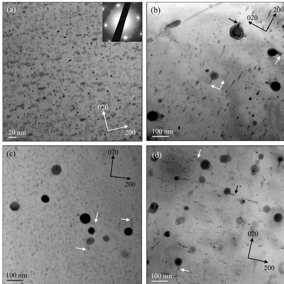
Fig. 3 Bright-field TEM images showing the precipitate microstructures in the T6 condition: (a) the base A alloy, (b) alloy B, (c) alloy E, and (d) alloy F
