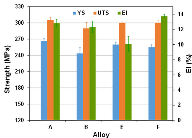
Fig. 6 Room-temperature tensile properties of 6082 alloys in the T6 condition
