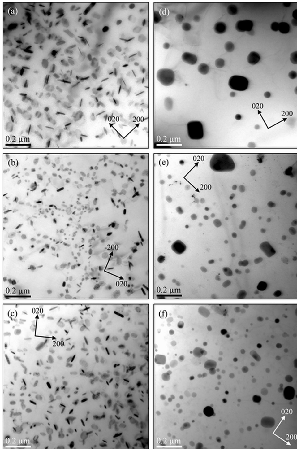
Fig. 2 Bright-field TEM images showing the dispersoid microstructures of alloys B (a, d), E (b, e) and F (c, f) in the as-homogenized (a, b, c) and T6A (d, e, f) conditions
