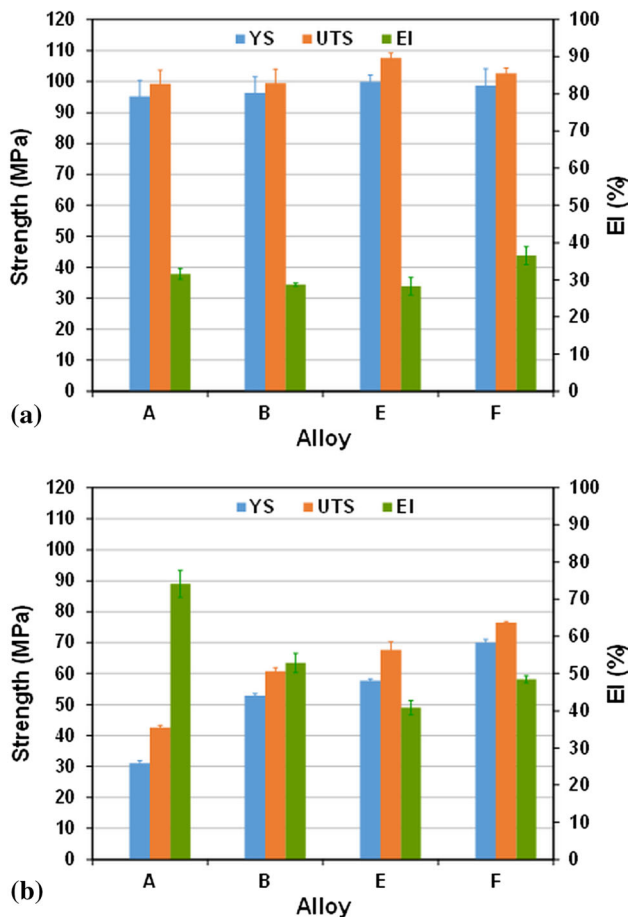
Fig. 7 Tensile properties of 6082 alloys at 300 °C in (a) T6 and (b) T6A conditions
