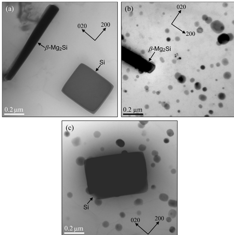
Fig. 4 Bright-field TEM images showing microstructures after thermal exposure at 300 °C for 100 h: (a) coarse \beta -Mg 2 Si and Si particles in the base A alloy, (b, c) relatively fine dispersoids beside coarse \beta -Mg 2 Si and Si particles in alloys E and F, respectively
