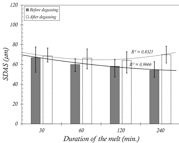
Fig. 6 Change in SDAS depending on holding time and degassing
