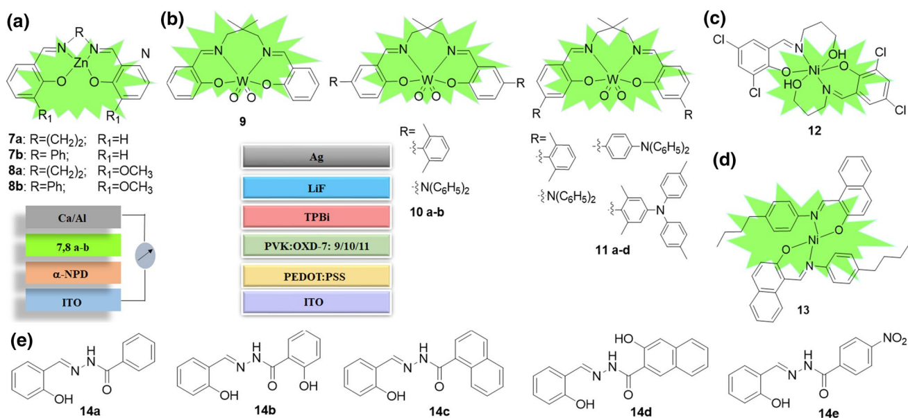
Fig. 5. Green emitting Schiff base complexes and their device architectures: (a) Zinc complexes with tetradentate Schiff bases (data from Ref. 76), (b) Tungsten Schiff bases with high QY and TADF (data
