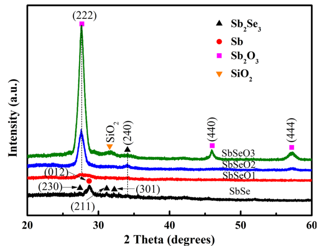
Fig. 4. XRD patterns of the SbSe and SbSeO x ( x = 1, 2, 3 ) films annealed at 300°C for 10 min in Ar Atmosphere.
