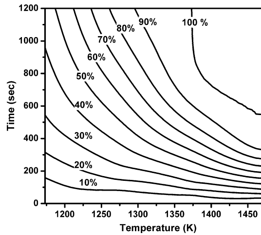
Fig. 5—Contour plot for iron formation as a function of temperature and time in a single 15 mm pellet. The pellet constitutes a mixture of hematite and carbon in a weight ratio of 1.5. The contour lines indicate the percentage of iron being produced.
