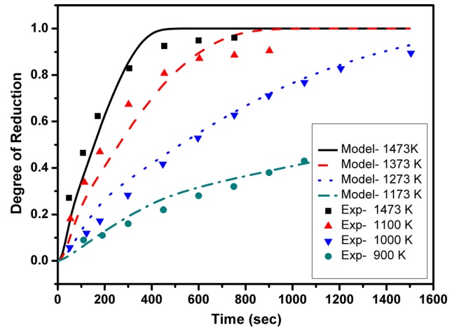
Fig. 3—Comparison between experimental and simulated results for different furnace temperatures for a single pellet for C/O ratio of 1.5 for a pellet of 15 mm diameter.
