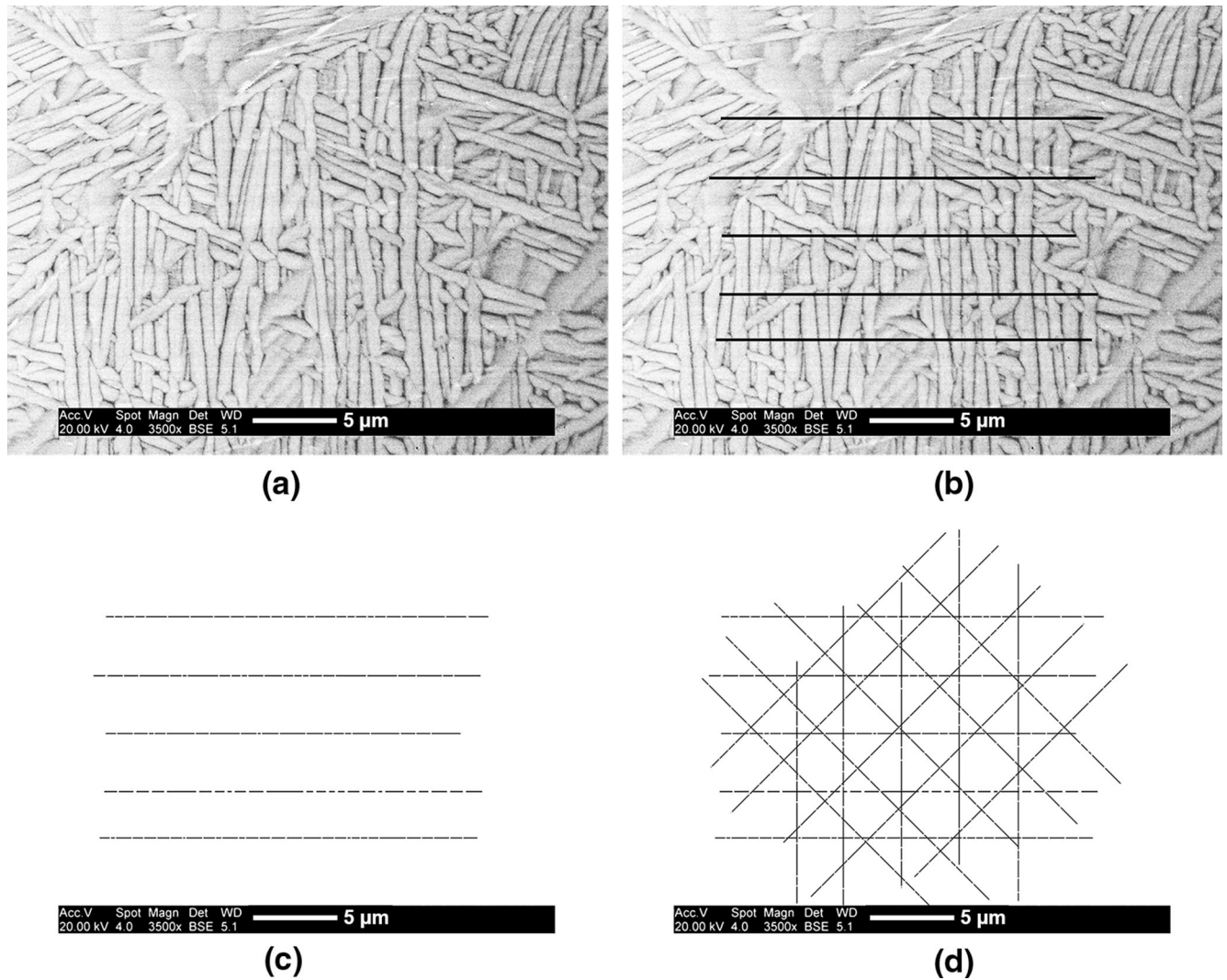
Fig. 2—Semi-automatic method to measure the thickness of the \alpha laths, as described in Tiley et al. [13] (a) shows as an example the original image taken from location C of the specimen rolled at 75 kN. (b) shows five lines of known length with 0 deg inclination. (c) shows the lines broken where they intercept \alpha phase boundaries. (d) shows the full set of lines oriented with 0, 45, 90, and 135 deg inclinations.
