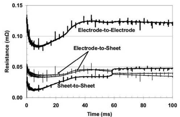
Fig. 13—Dynamic resistance curves of sample made at 2700 A.
