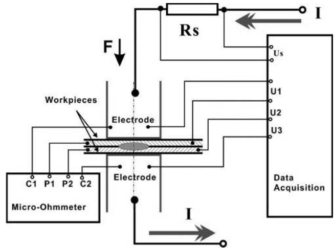
Fig. 2—Experimental setup.
