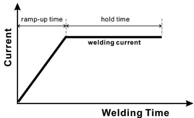
Fig. 3—Current waveform.
