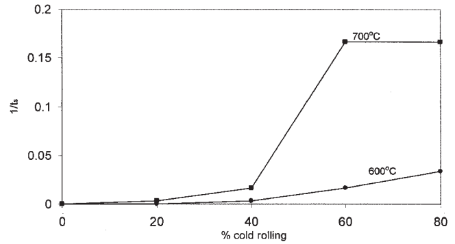
Fig. 2—Variation in desensitization time at different temperatures with degree of cold rolling.
