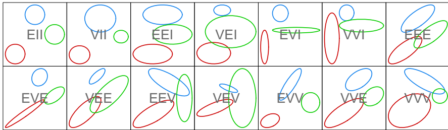
Fig. 2 Ellipses of isodensity for each of the 14 parsimonious eigen-decomposition covariance parameterisations for multivariate data in GPCMs, with three components in two dimensions
