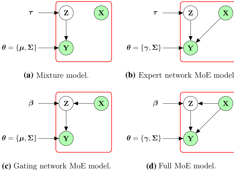
Fig. 1 The graphical model representation of the mixture of experts models. The differences between the special cases are due to the presence or absence of edges between the covariates \mathbf{X} and the latent variable \mathbf{Z} and/or response variable \mathbf{Y} . Note that different subsets of the covariates in \mathbf{X} can enter these two different parts of the full MoE model in (d)
