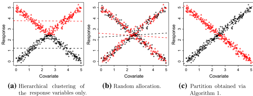
Fig. 3 Initial 2-component partitions on univariate data clearly arising from a mixture of two linear regressions, obtained using a agglomerative hierarchical clustering, b random allocation, and c Algorithm 1 applied to the initialisation in (b) , demonstrating the improvement achieved by incorporating expert network covariates into the initialisation strategy. Allocations are distinguished using black points and red triangles. Corresponding fitted lines are also shown
