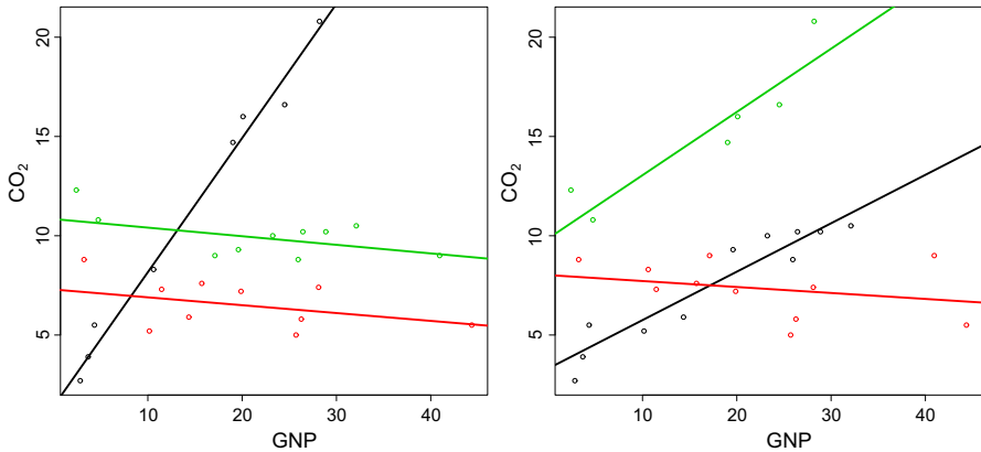
(a) With Algorithm 1 invoked for initialisation, achieving a BIC value of -155.20 .
