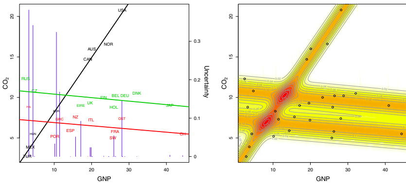
(a) Fitted lines of the expert network GLMs. Text label size is proportional to a country’s probability of belonging to its assigned cluster. Clustering uncertainty is also indicated by vertical bars relating to the second y-axis.
