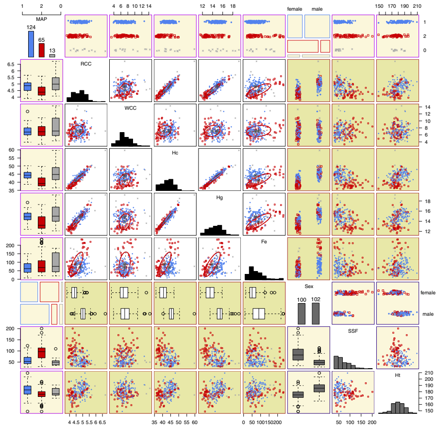
Fig. 5 Generalised pairs plot for the optimal MoEClust model fit to the AIS data, depicting pairwise relationships between the hematological response variables, the expert network covariate Sex, the gating concomitants SSF and Ht, and the MAP classification. Colours and plotting symbols correspond to the MAP classification: blue circles and red squares for the two Gaussian clusters; grey crosses for the 4 female and 9 male outlying observations assigned to the uniform noise component. Mosaic plots are used to depict two categorical variables, scatter plots are used for panels involving two continuous variables, and a mix of box-plots and jittered strip-plots are used for mixed pairs (colour figure online)
