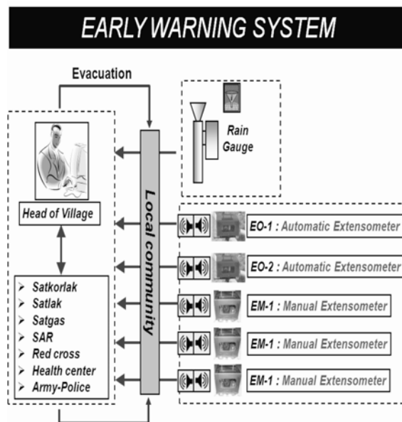
Figure 9 Integration of technical and social system of landslide early warning and disaster risk reduction in Ledokasari Village, Karanganyar Regency, Indonesia (Karnawati et al. 2009 and Karnawati et al. 2010).
