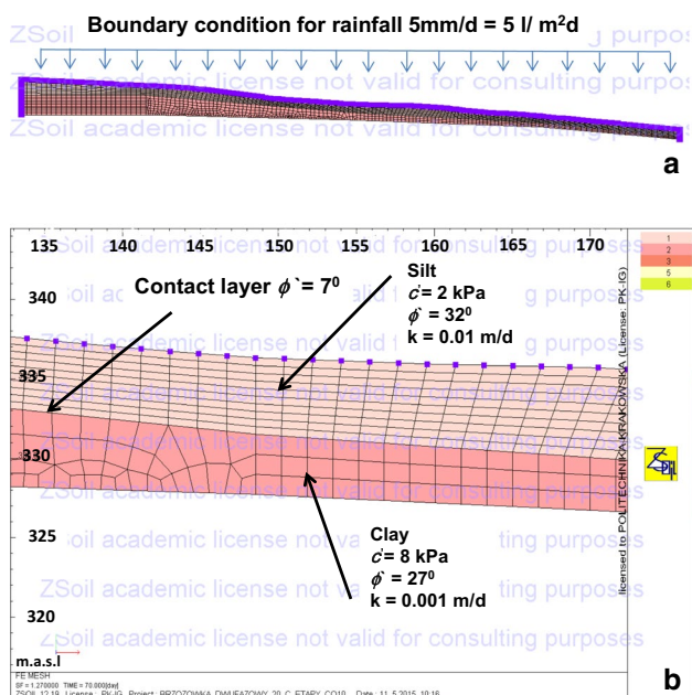
Fig. 8 Numerical model— a overview, b detailed view
