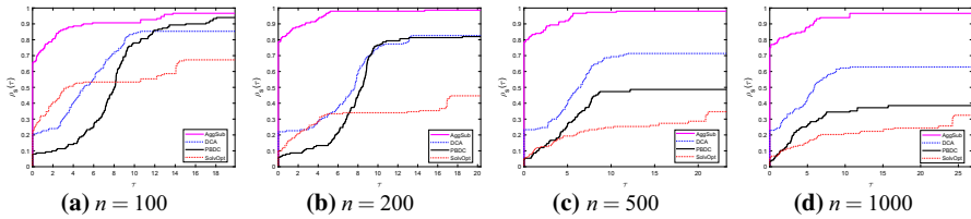
Fig. 1 CPU time
