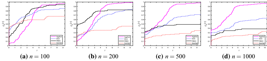
Fig. 2 Number of subgradient evaluations
