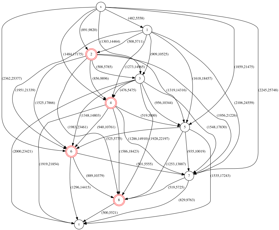
Fig. 1 Example instance with (|N|, m) = (10, 2)
