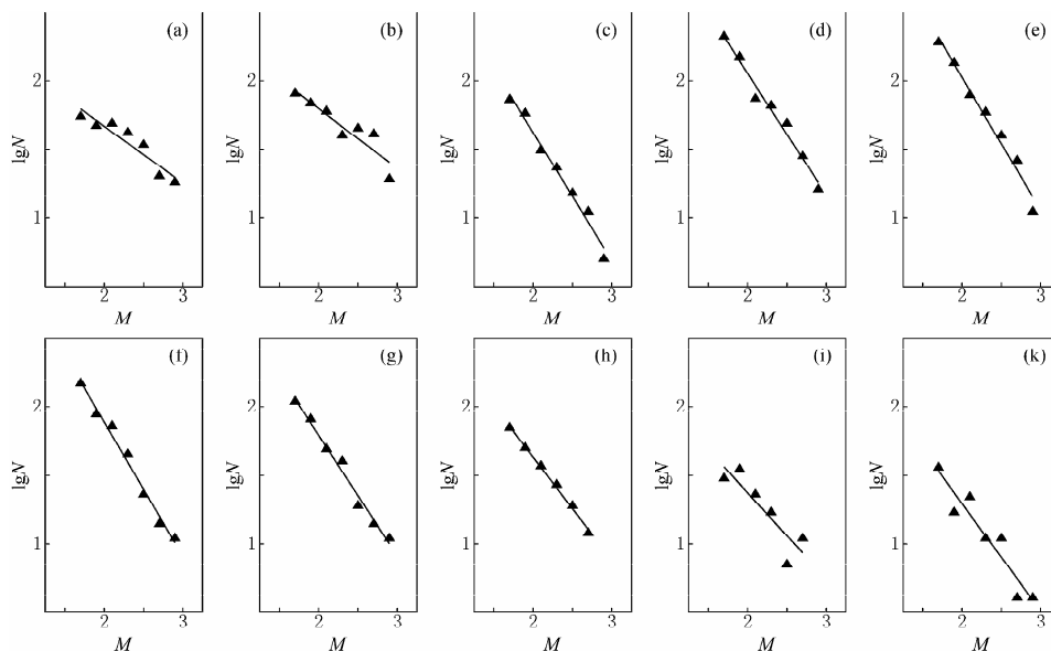
Figure 5 Frequency-magnitude relation ( b -values) at different depths beneath the study area. The lines are regressed from frequency-magnitude points. The depth is in the range of 0 to 20 km with interval of 2 km from (a) to (k), respectively.
