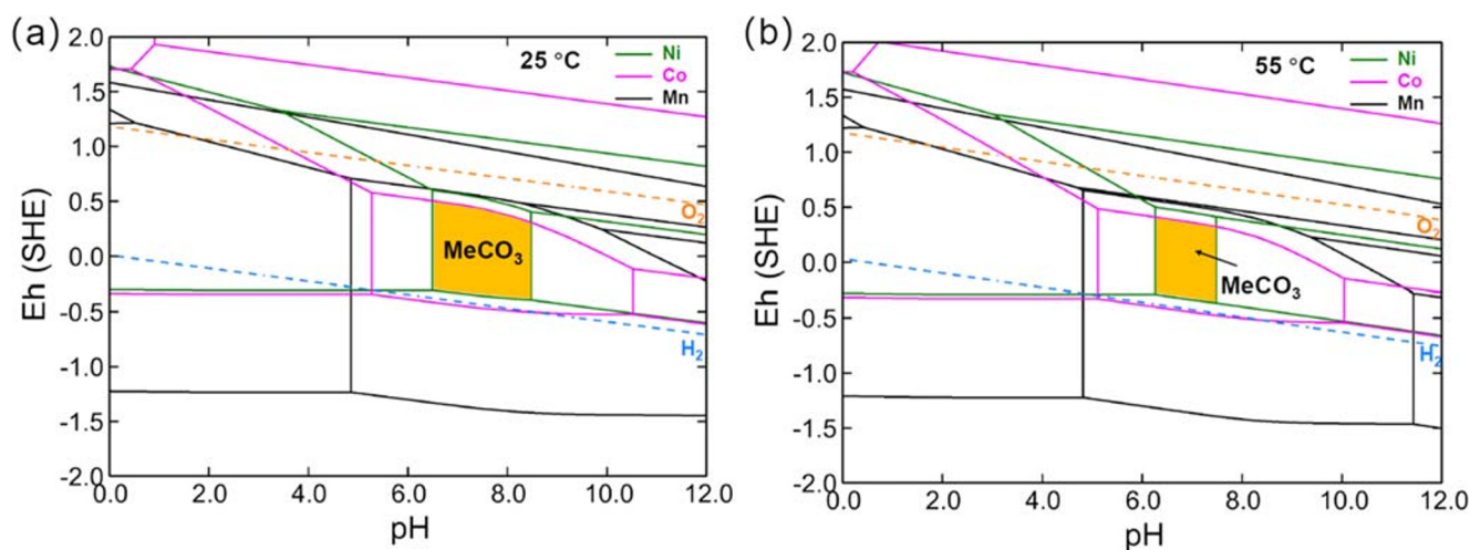
Fig. 4 Eh-pH simulations for the synthesis of \text{Ni}_{0.13}\text{Co}_{0.13}\text{Mn}_{0.54}(\text{CO}_3)_{0.8} at (a) 25 °C and (b) 55 °C (where [\text{Ni}^{2+}] = 0.13 \text{ mol kg}^{-1} , [\text{Co}^{2+}] = 0.13 \text{ mol kg}^{-1} , and [\text{Mn}^{2+}] = 0.54 \text{ mol kg}^{-1} )
