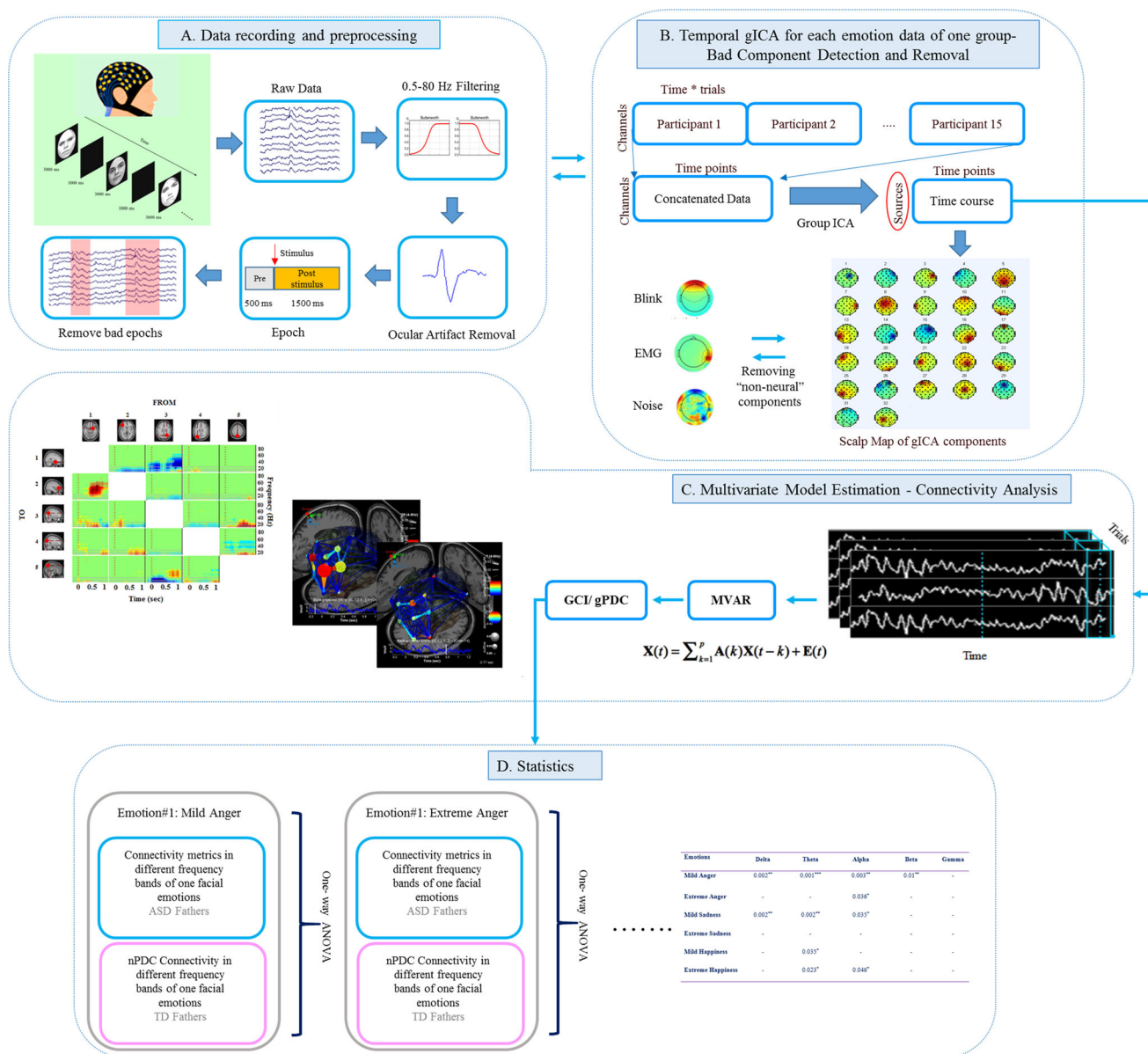
Fig. 2 Summary of EEG data analysis pipeline. a Steps of all preprocessing procedures. b Temporal group ICA: Concatenating EEG data of specified emotion corresponding to all participants of one group temporally and then applying ICA. Eliminating “non-neural” components like muscle activity, eye blink, line noise based
