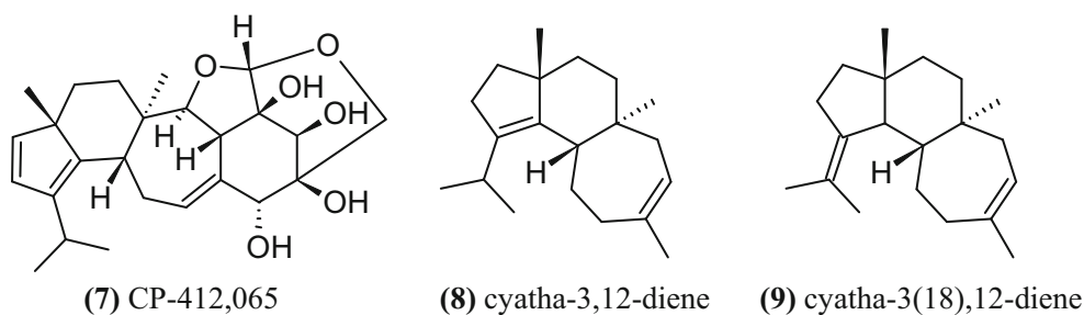
Fig. 3 Chemical structures of selected cyathane diterpenoids from submerged cultures of H. erinaceus
