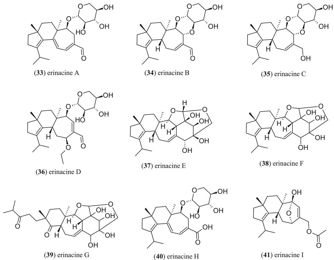
Fig. 8 Chemical structures of erinacines and other cyathane diterpenes with neuroprotective effects from H. erinaceus (Part 1)
