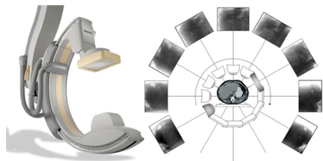
Fig. 1 CBCT imaging is based on the rotation of a C-arm equipped with a flat panel detector ( left image ) around the patient. 2D projections are acquired ( right image ) and reconstructed to generate a 3D volumetric data set
