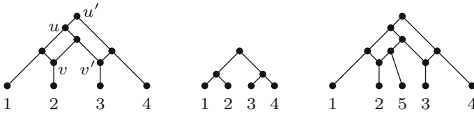
Fig. 2 Left A phylogenetic network \mathcal{N} that displays three trees. Middle A phylogenetic tree that is displayed twice by \mathcal{N} . Right A phylogenetic network \mathcal{N}' that displays four trees. While \mathcal{N} and \mathcal{N}' are both tree-sibling, only \mathcal{N}' also satisfies the stronger tree-child condition
